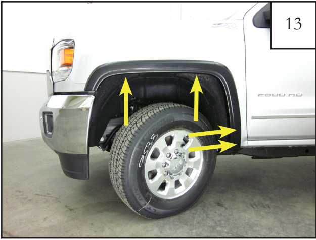
13 While holding Flare on vehicle, install supplied screw (SW1-0056) into the four factory hole locations as shown. Do not fully tighten at this time.
