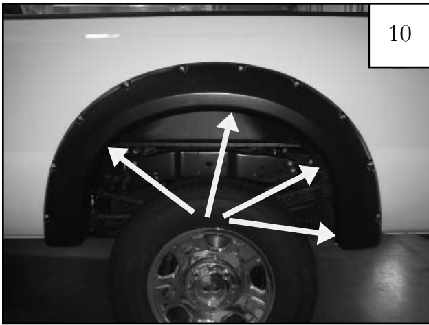
Clip locations. Use holes in flare to mark the four clip locations.
