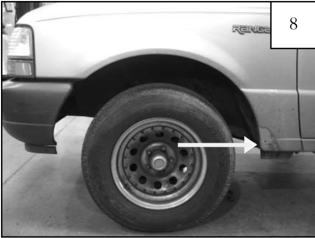
Remove factory screw at rear of wheel well. Save for reinstallation.
