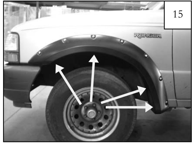
Ensuring proper flare placement, tighten all screws.
