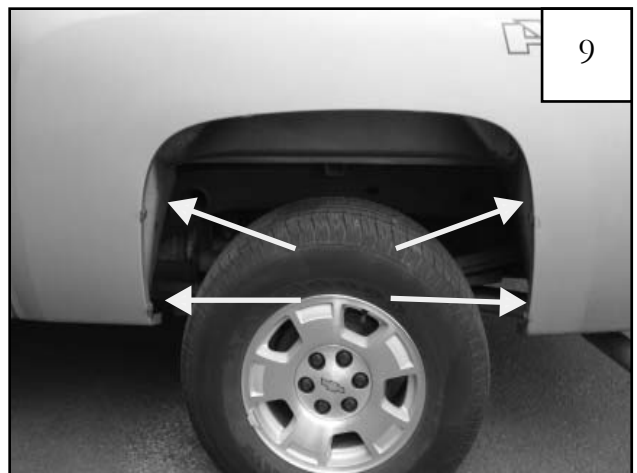
Slide a supplied Clip (CL1-0005) over lower four tabs. Clips may need to be adjusted to align with holes in flare.
