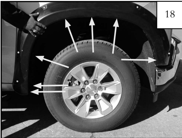
Press flare firmly against body and tighten all screws.
