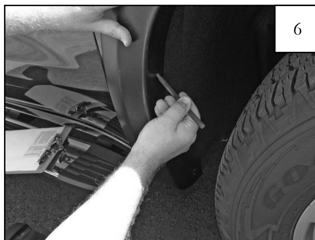
Use a grease pencil to mark the two locations of the holes indicated with the circles in Step 5. Remove flare from vehicle.
