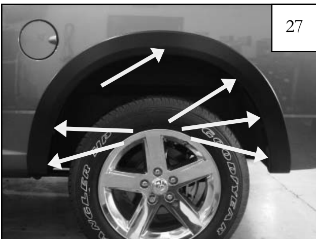
Supplied screw locations. Install one supplied screw at the top of flare first for easier installation. See step 28.
